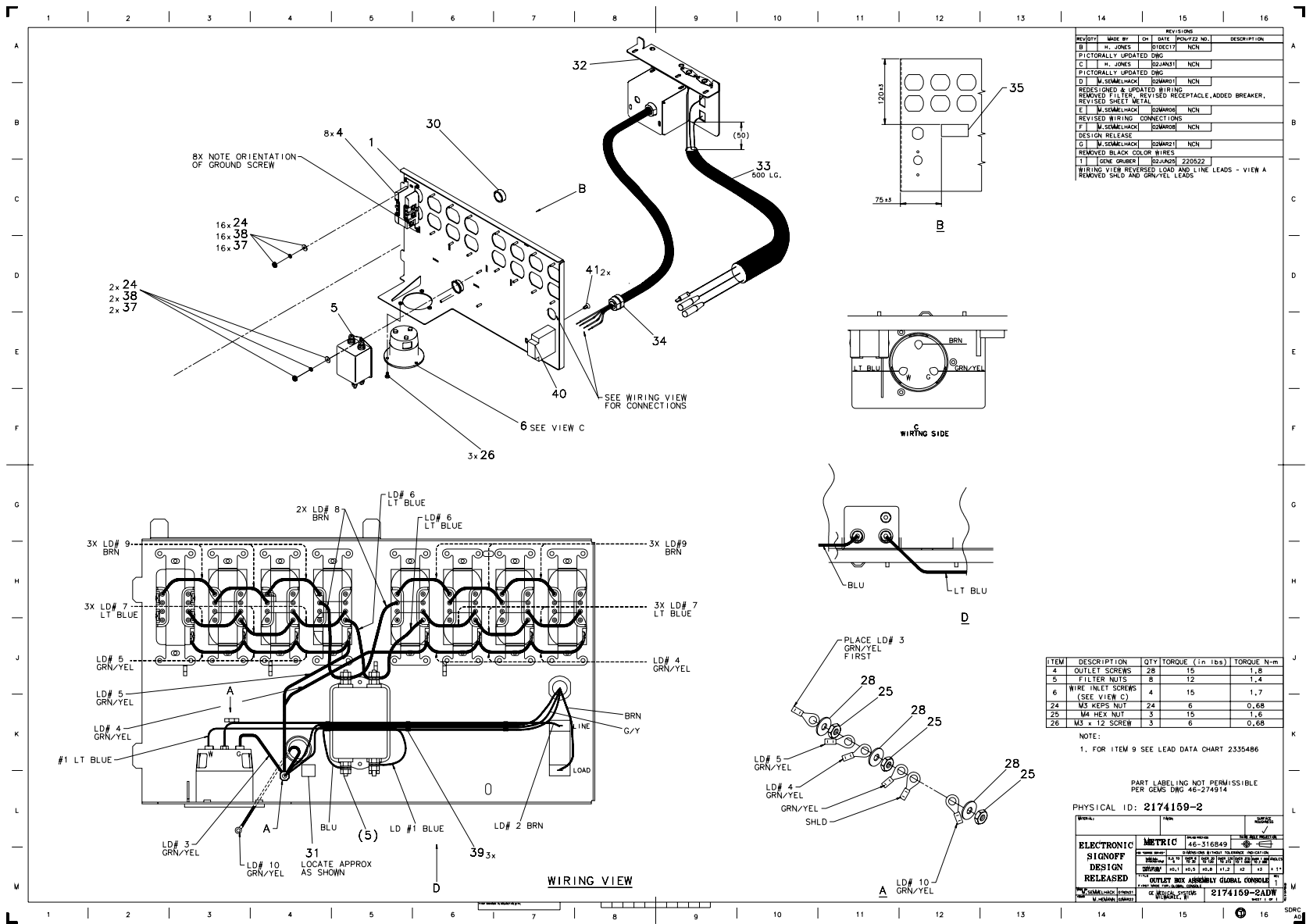
Figure 6-23 Outlet Box Assembly (2174159-2, sheet 1, rev 1)
