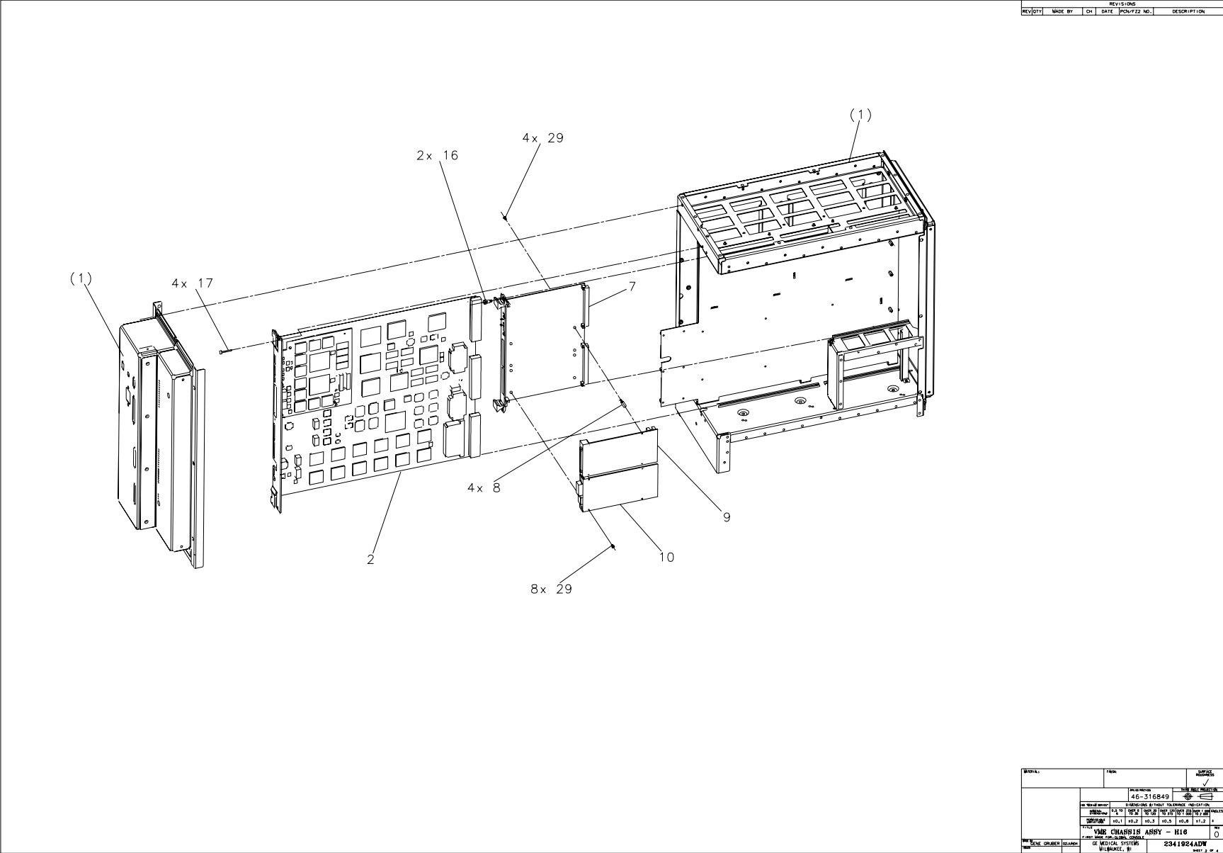
Figure 6-10 Recon Box Assembly (2341924, sheet 2, rev 0)
