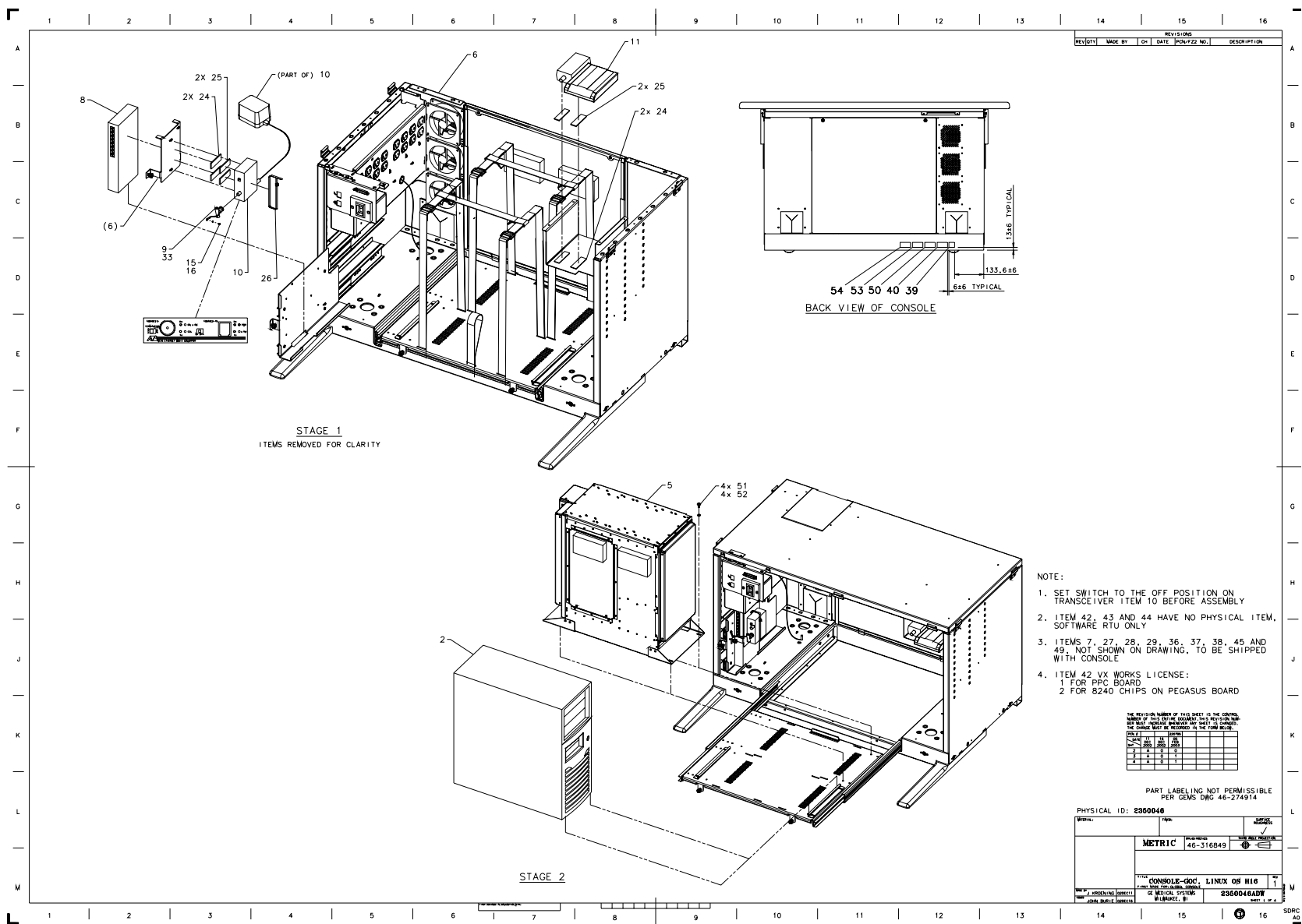
Figure 6-3 Console Assembly (2350046, sheet 1, rev 1)
