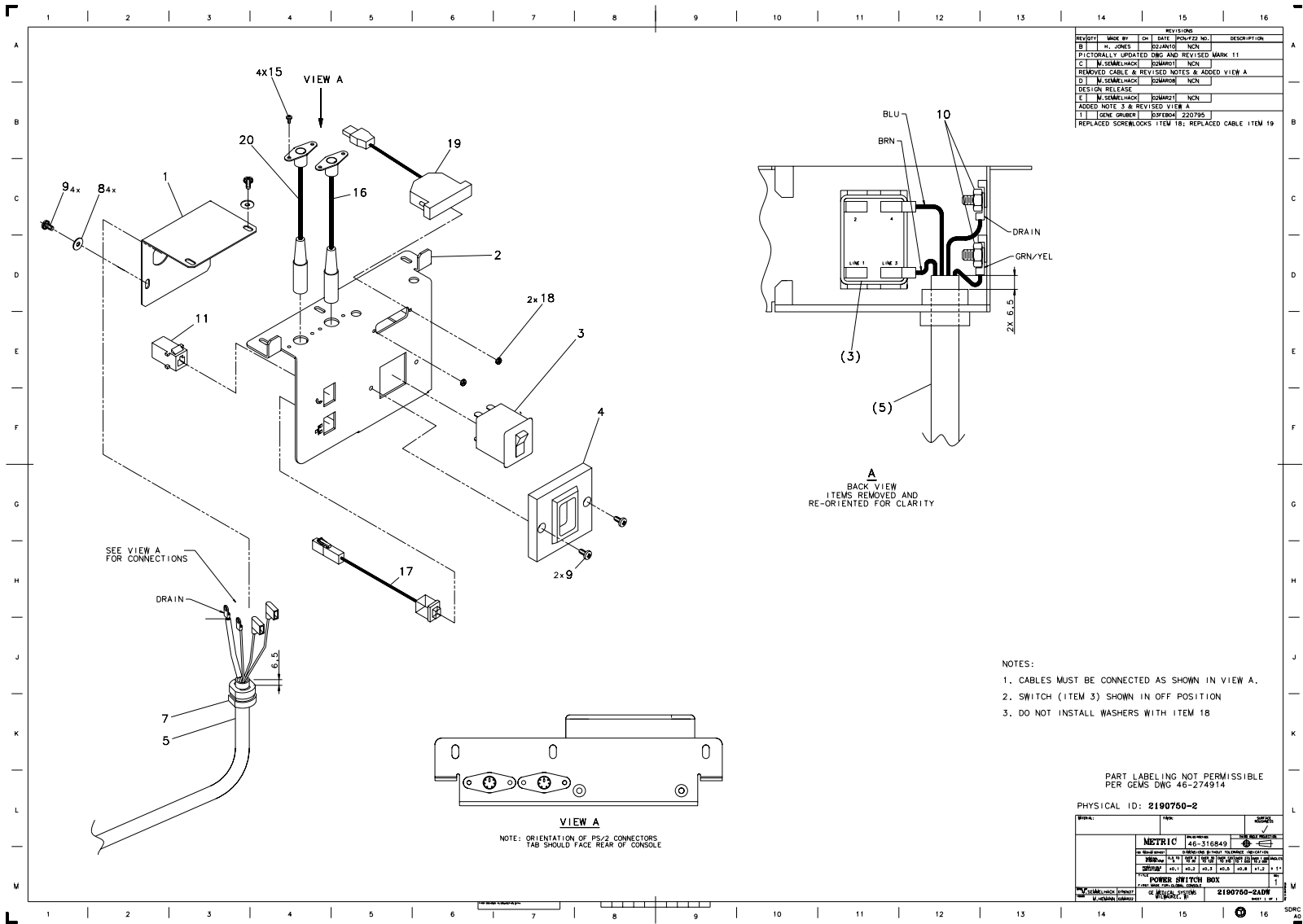
Figure 6-24 Power Switch Box (2190750-2, sheet 1, rev 1)
