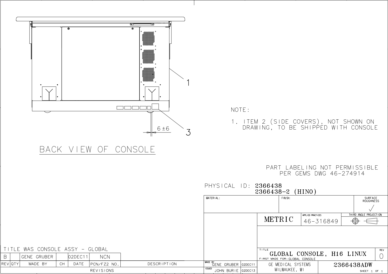
Figure 6-2 Global Console Assembly (2366438, sheet 1, rev 0)
