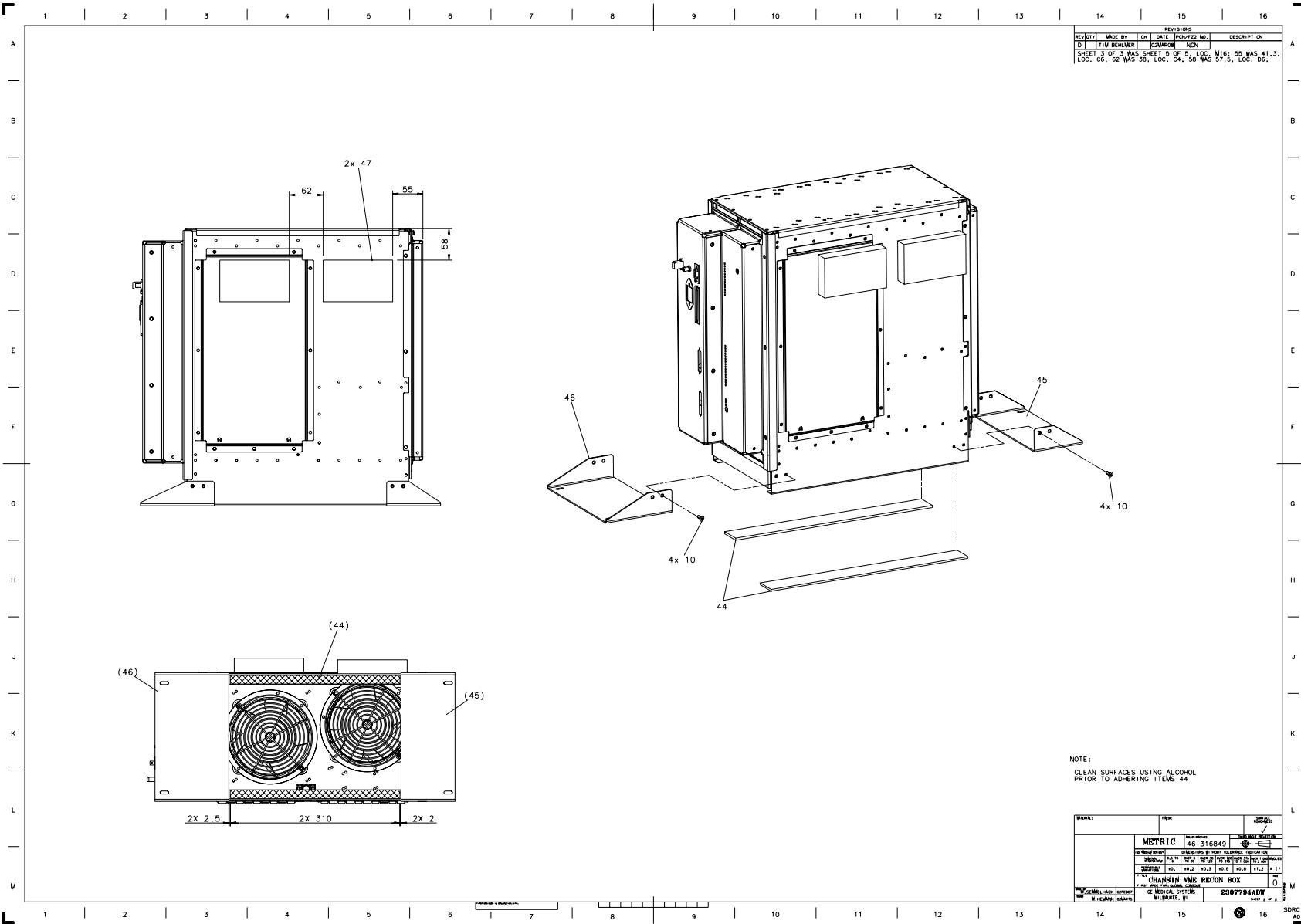
Figure 6-20 VME Chassis Assembly (2307794, sheet 3, rev 0)
