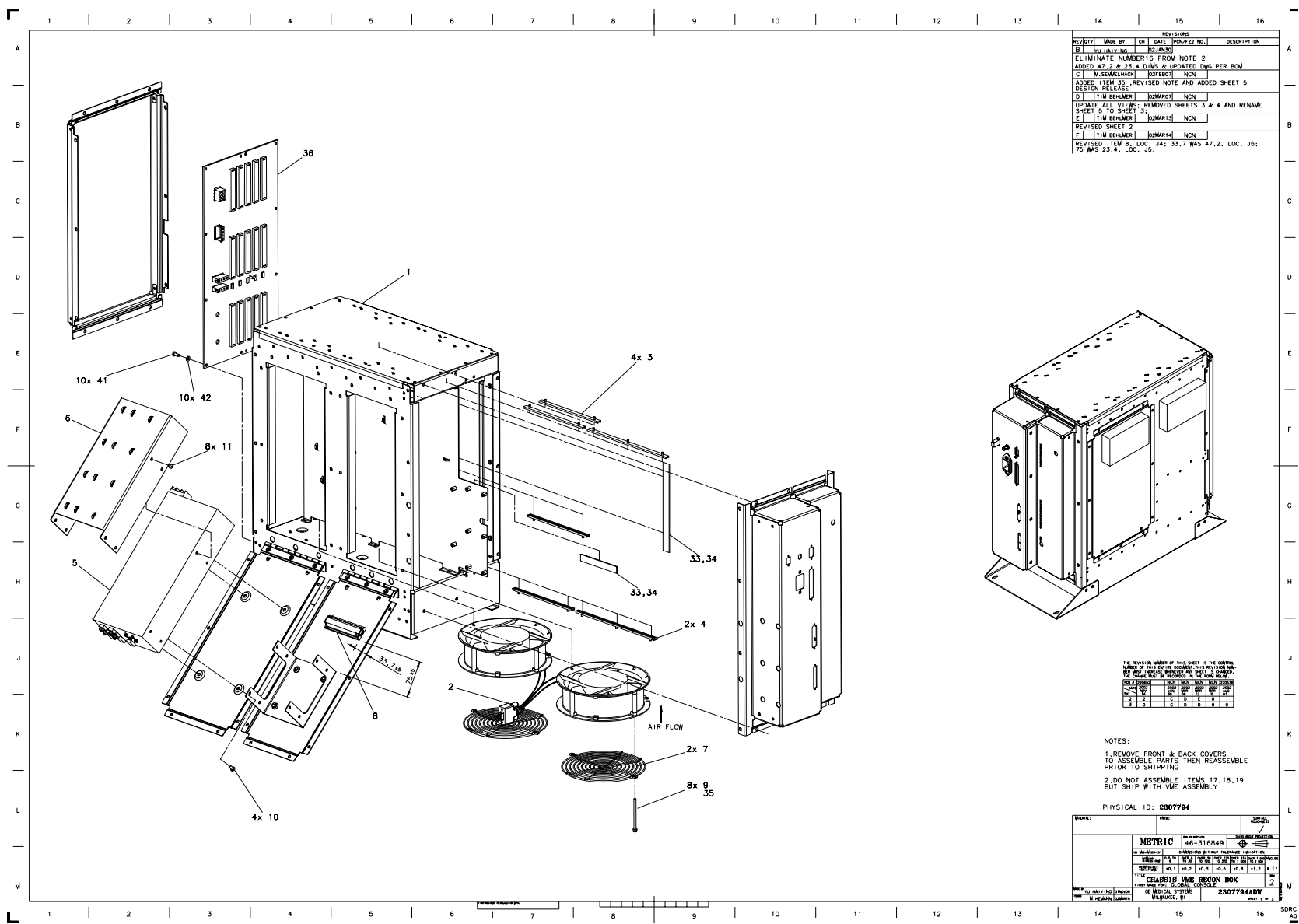
Figure 6-18 VME Chassis Assembly (2307794, sheet 1, rev 2)
