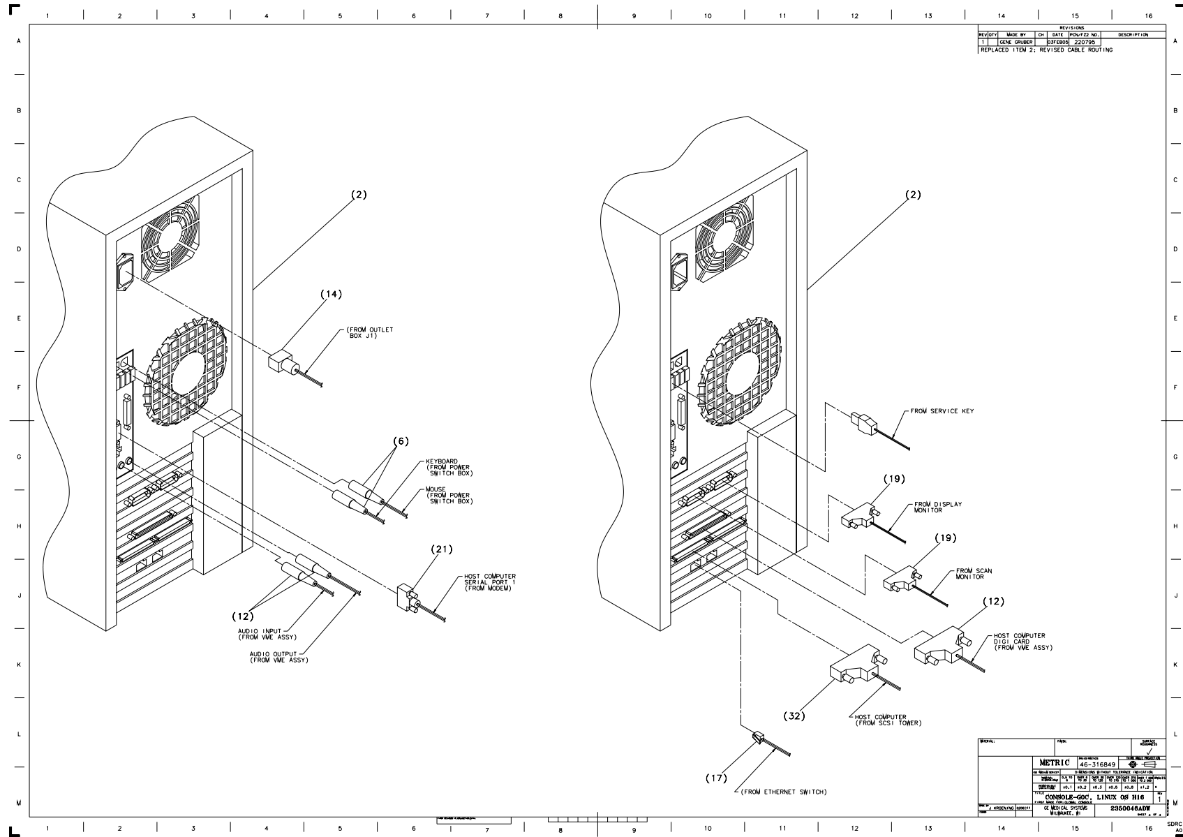
Figure 6-6 Console Assembly (2350046, sheet 4, rev 1)
