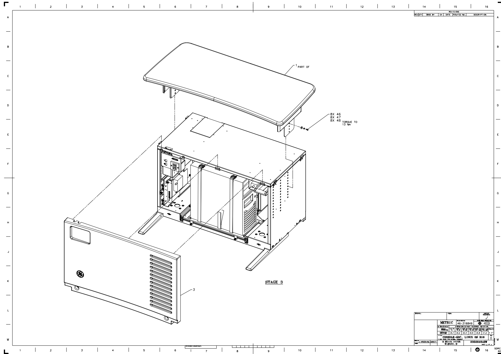
Figure 6-4 Console Assembly (2350046, sheet 2, rev 0)
