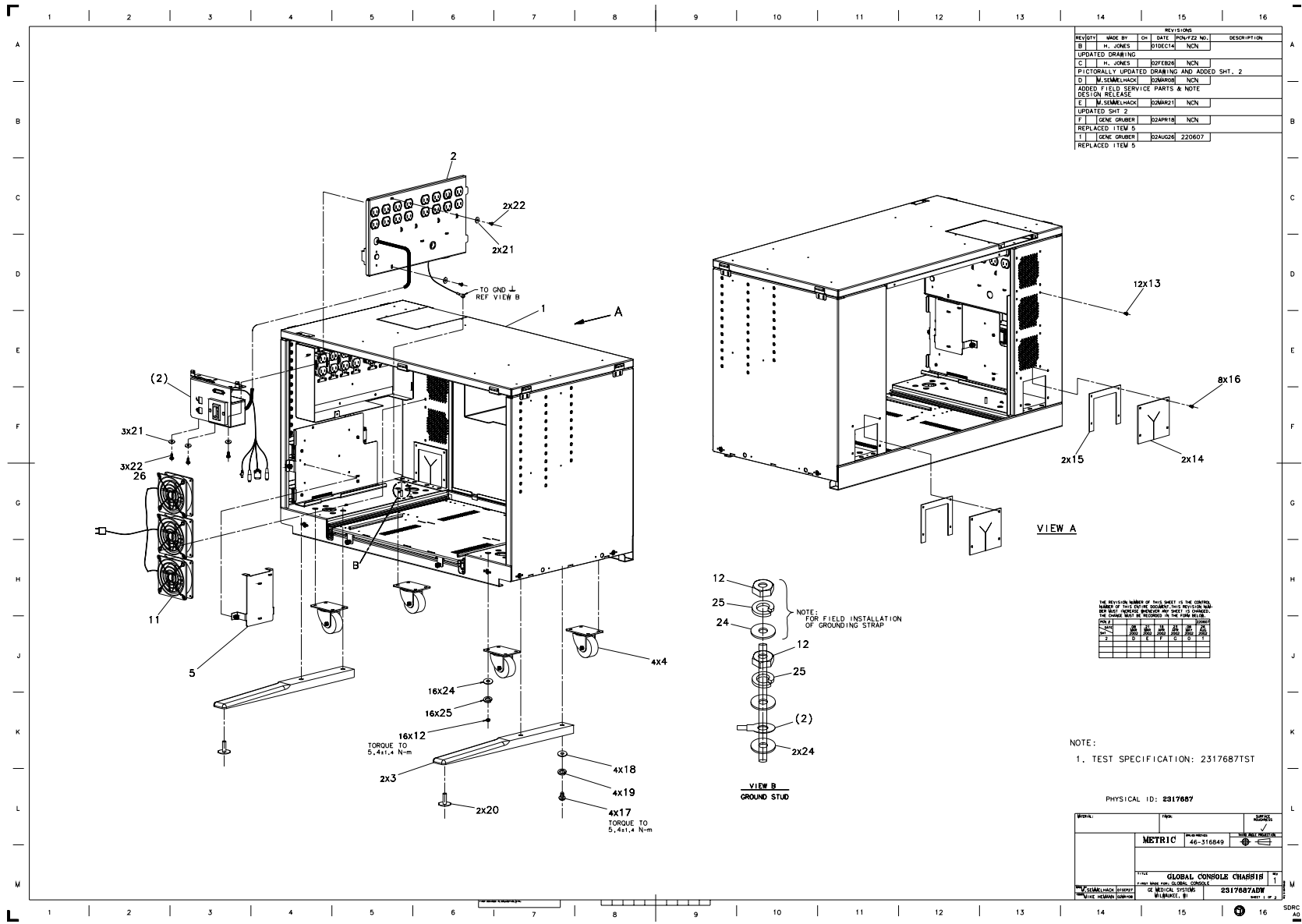
Figure 6-26 Console Chassis Assembly (2317687, sheet 1, rev 1)
