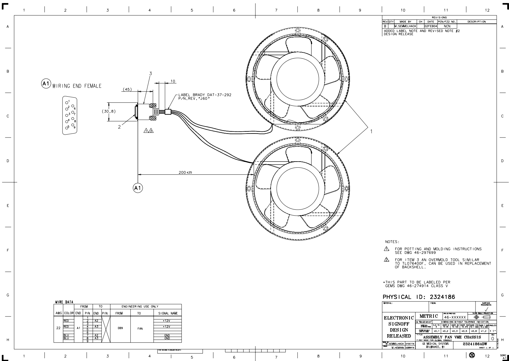
Figure 6-16 Fan Assembly, VME Chassis (2324186, sheet 1, rev 0)
