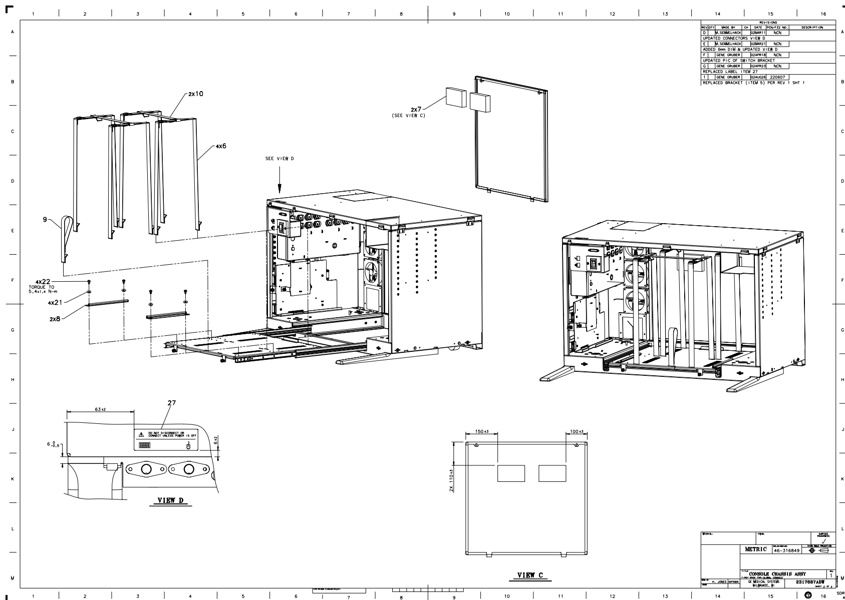
Figure 6-27 Console Chassis Assembly (2317687, sheet 2, rev 1)
