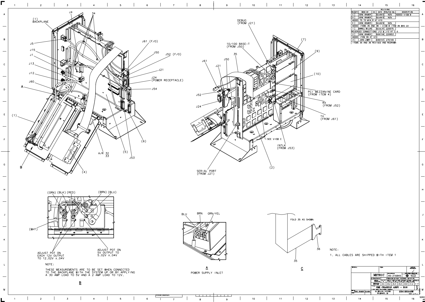
Figure 6-11 Recon Box Assembly (2341924, sheet 3, rev 3)
