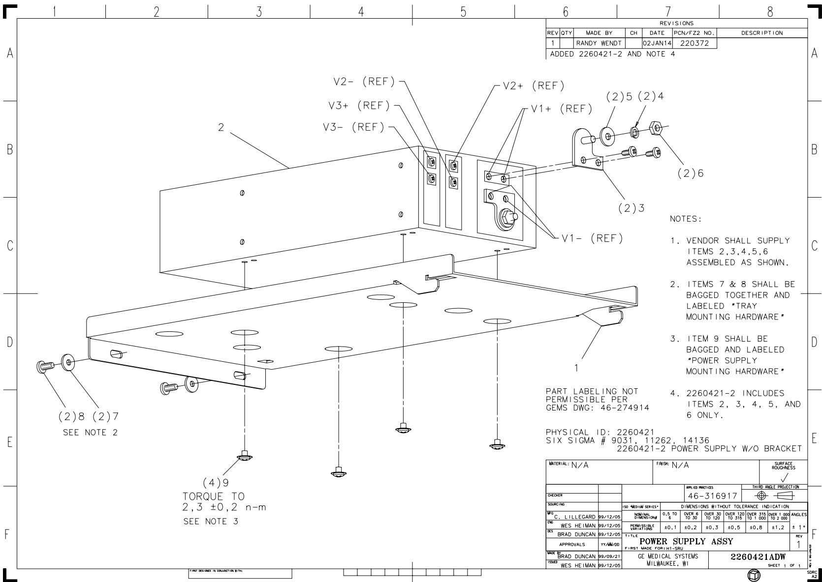
Figure 6-17 VME Console Power Supply (2260421, sheet 1, rev 1)
