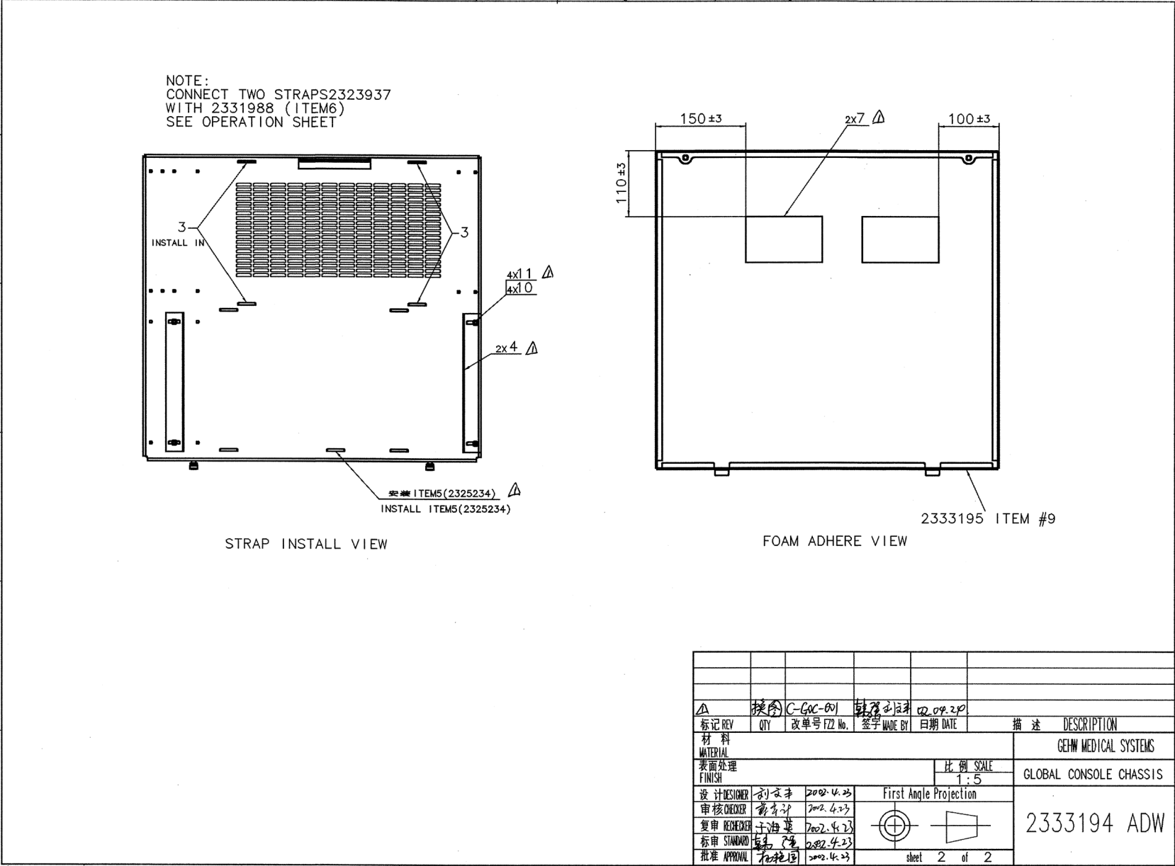
Figure 6-22 Console Chassis Assembly (2333194 sheet 2, rev 1)
